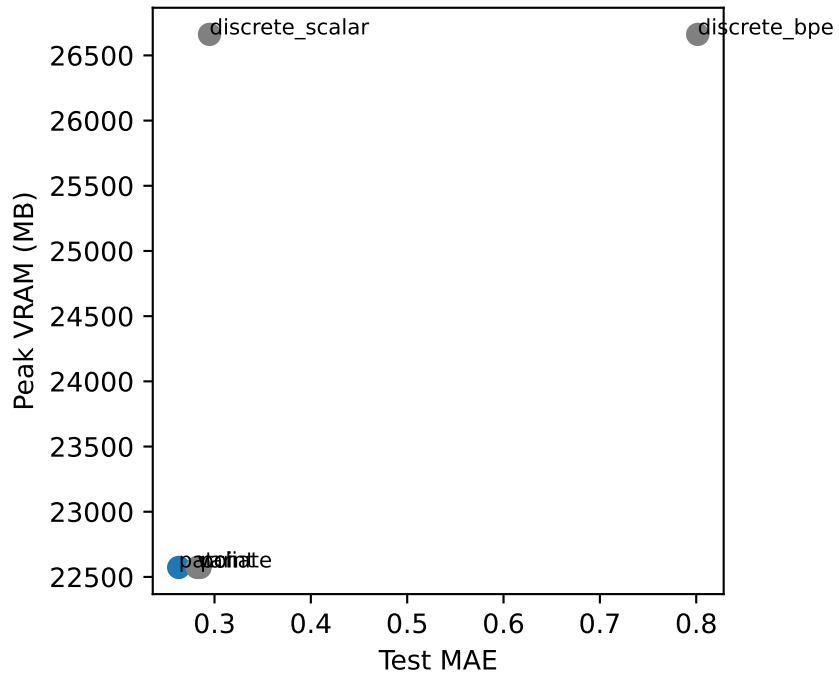
Electricity/H=336: MAE vs. VRAM
