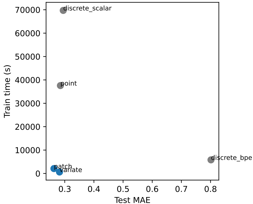
Electricity/H=336: MAE vs. time
