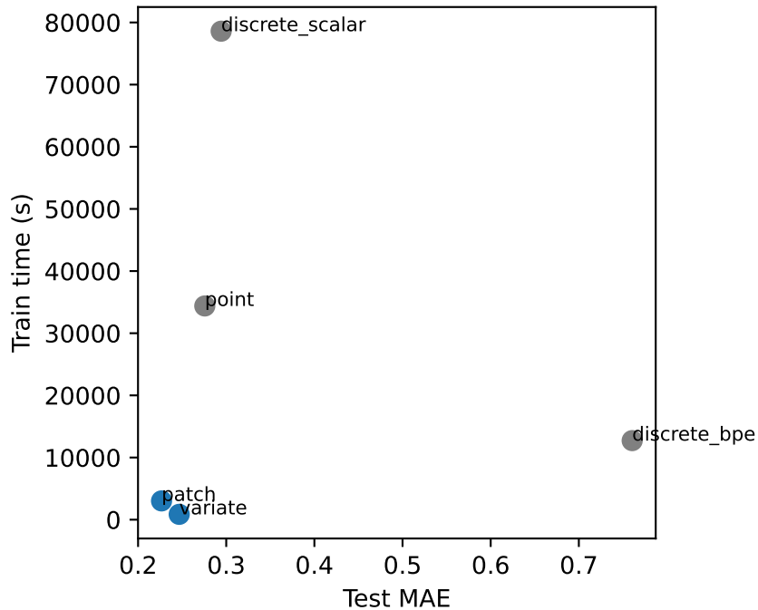
Electricity/H=96: MAE vs. time
