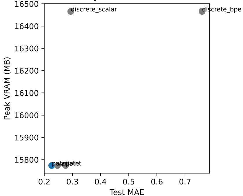
Electricity/H=96: MAE vs. VRAM
