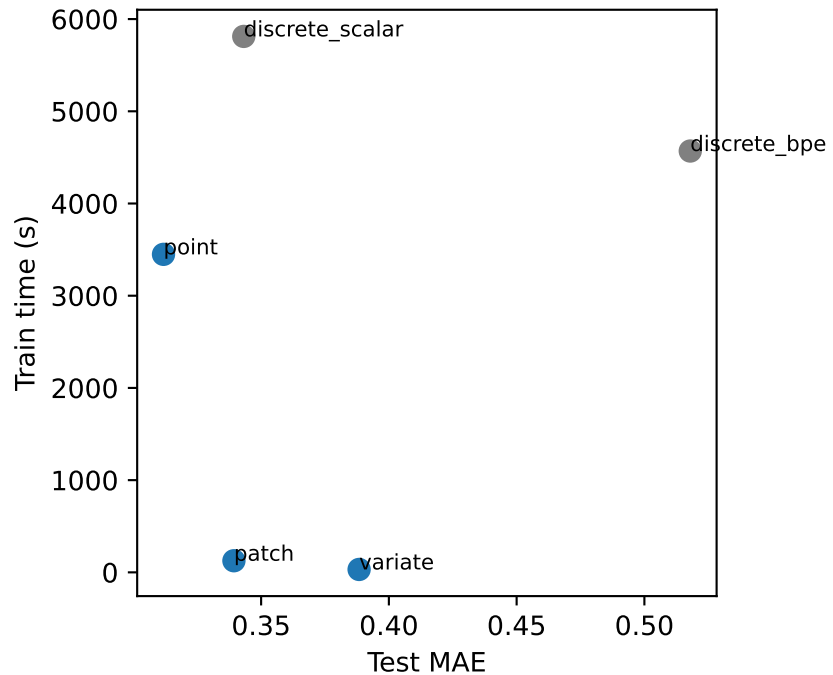
Weather/H=336: MAE vs. time
