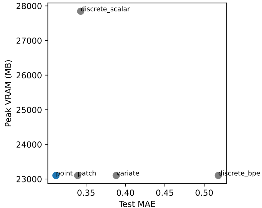
Weather/H=336: MAE vs. VRAM
