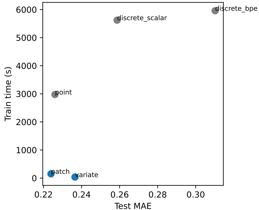
Weather/H=96: MAE vs. time
