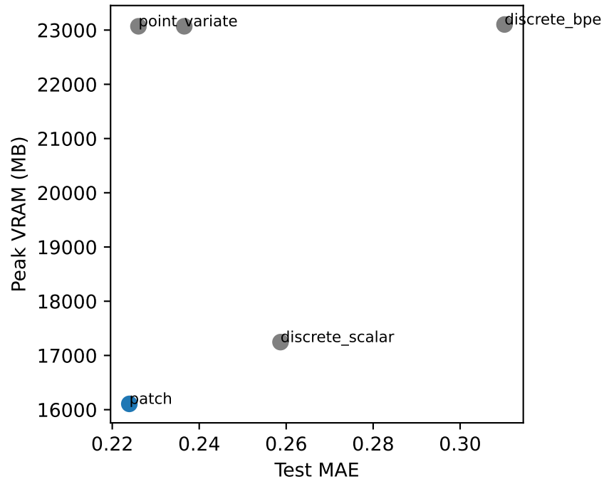
Weather/H=96: MAE vs. VRAM
