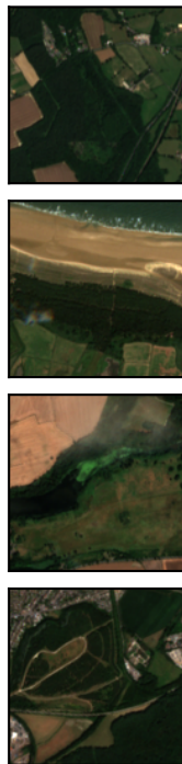
Sentinel-2 RGB
