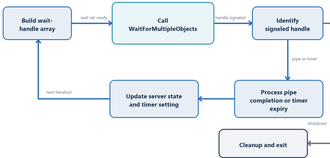
Figure 4. Main server wait-set construction and dispatch
