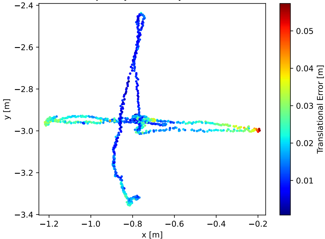
Estimated Trajectory Colored by Translational Error
