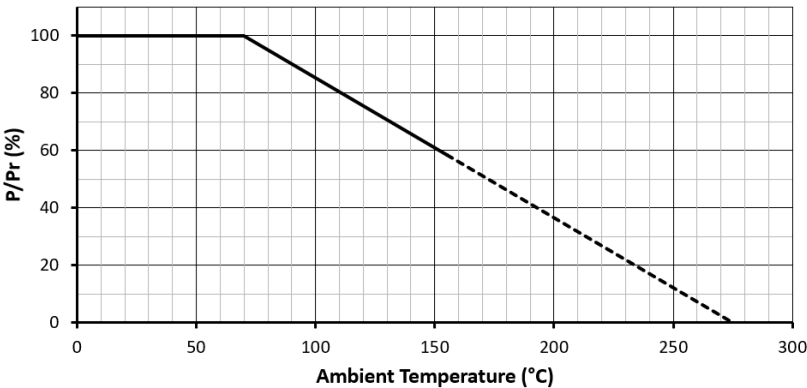
Temperature Derating
