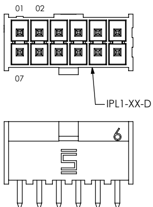
FIG 8 (IPL1-106-02-XXX-D-TR SHOWN) (MUST USE K-DOT-.256-.375-.005) (DIFFERENT AS SHOWN, OTHERWISE SAME AS FIG 2)
