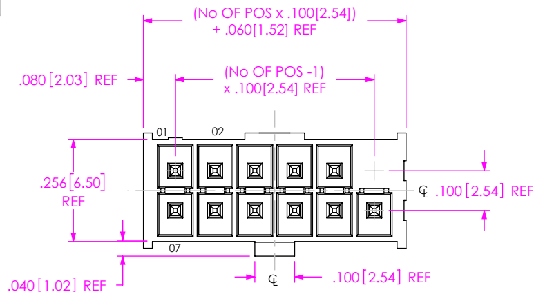
FIG 1 IPL1-106-01-XXX-D-P SHOWN
