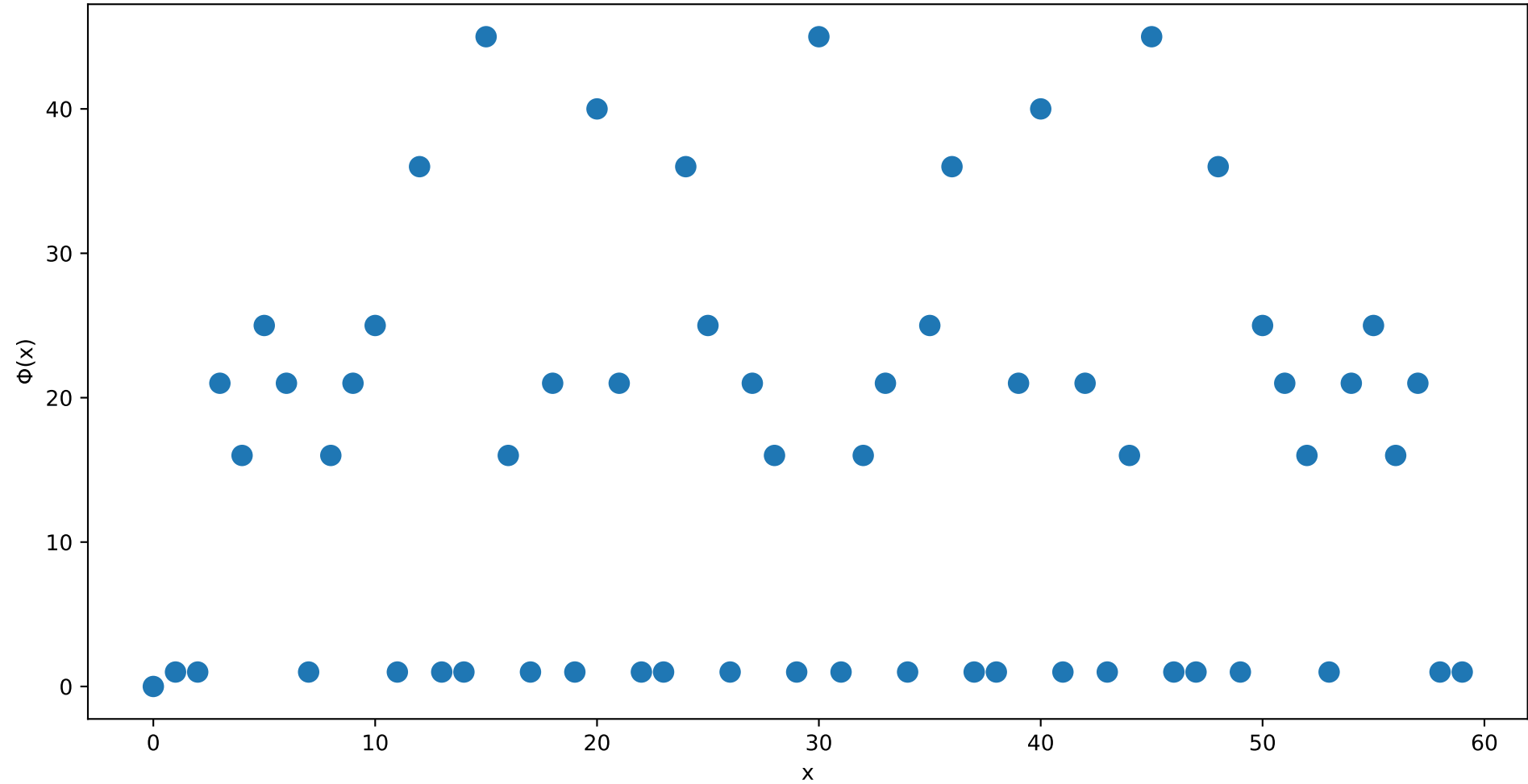
MDST — \Phi Field over Z60
