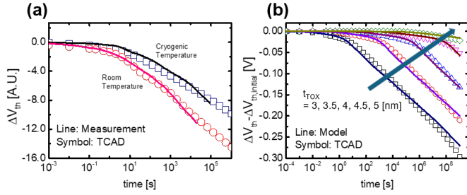
Fig. 3. (a) The TCAD simulation calibration with the measurement from previous study [2]. (b) A detail detrapping curve variation over time with t_{ox} from 3 nm to 5 nm.
