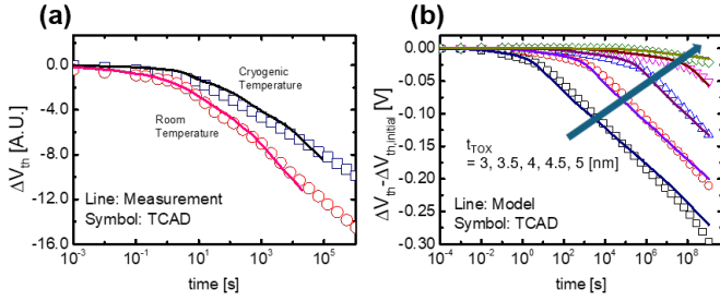
Fig. 3. (a) The TCAD simulation calibration with the measurement from previous study [2]. (b) A detail detrapping curve variation over time with t_{\text{TOX}} from 3 nm to 5 nm.
