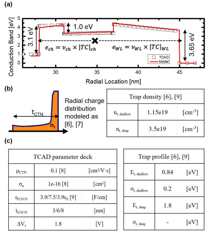
Fig. 2. (a) The band diagram with barrier notations where detrapping of trapped electron occurs, (b) a detail programmed trapped charge distribution after program operation, and (c) TCAD parameter deck and used trap profile within the simulation [6]–[9].
