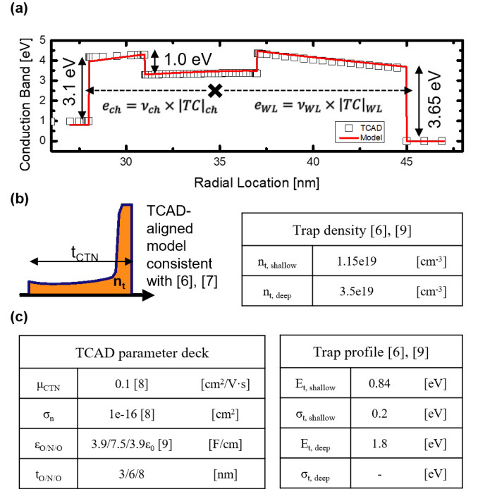
Fig. 2. (a) The band diagram with barrier notations where detrapping of trapped electron occurs, (b) a detail programmed trapped charge distribution after program operation the TCAD-aligned modeled radial trapped-charge profile [6], [7] used as the initial condition of the time-step-free model, and (c) TCAD parameter deck and used trap profile within the simulation [6]–[9].
