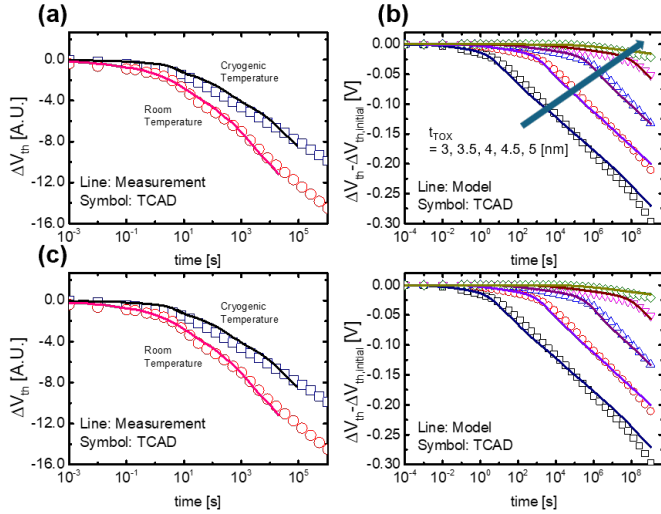
Fig. 3. (a) The TCAD simulation calibration with the measurement from previous study [2]. (b) A detail detrapping curve variation over time with t_{TOX} from 3 nm to 5 nm.
