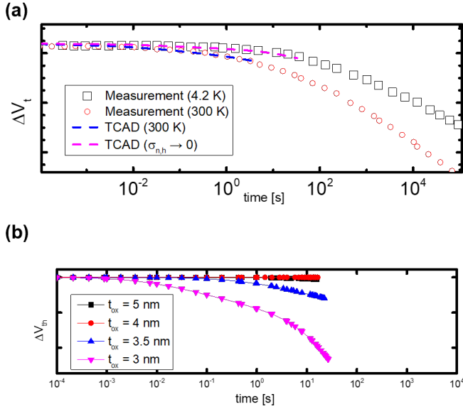
Fig. 2. (a) The TCAD simulation calibration with the measurement from previous study [2]. (b) A detail detrapping curve variation over time with t_{tox} from 3 nm to 5 nm.
