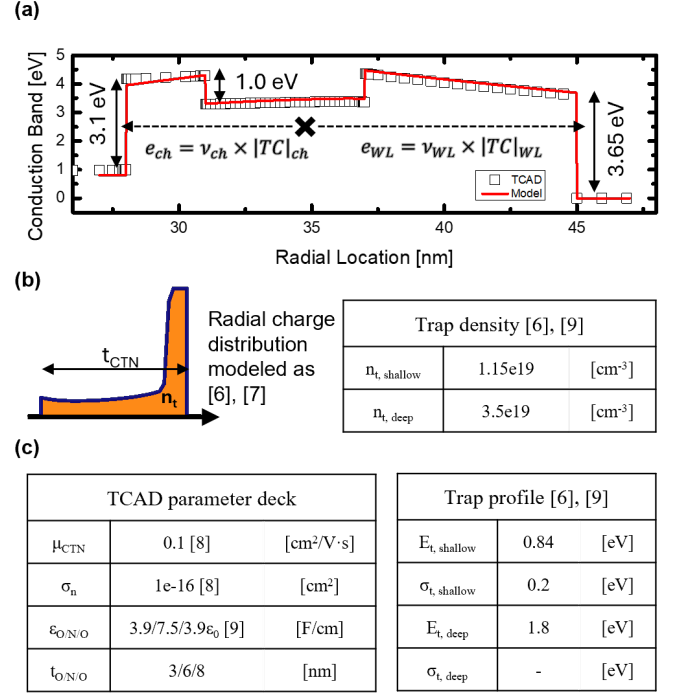
Fig. 2. (a) The band diagram with barrier notations where detrapping of trapped electron occurs, (b) a detail programmed trapped charge distribution after program operation, and (c) TCAD parameter deck and used trap profile within the simulation [6]–[9].
