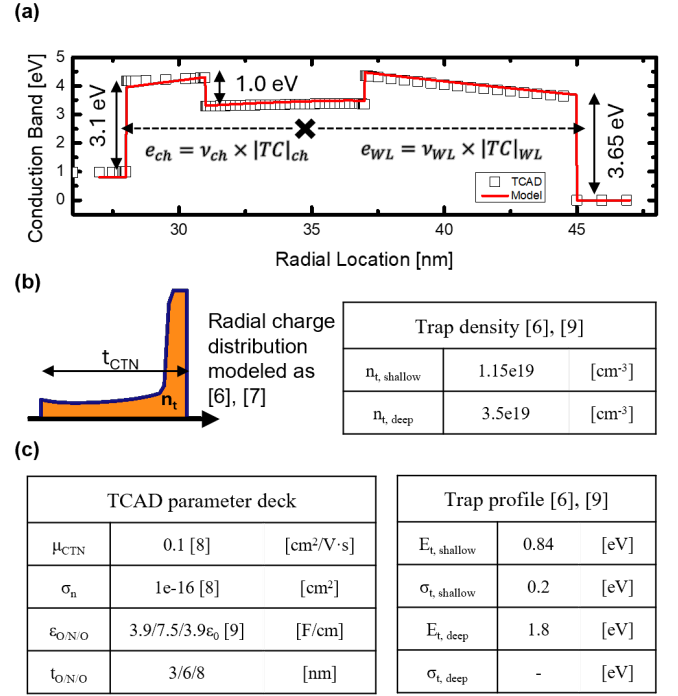
Fig. 2. (a) The band diagram with barrier notations where detrapping of trapped electron occurs, (b) the radial trapped charge distribution used as the model initial condition, and (c) TCAD parameter deck and used trap profile within the simulation [6]–[9].
