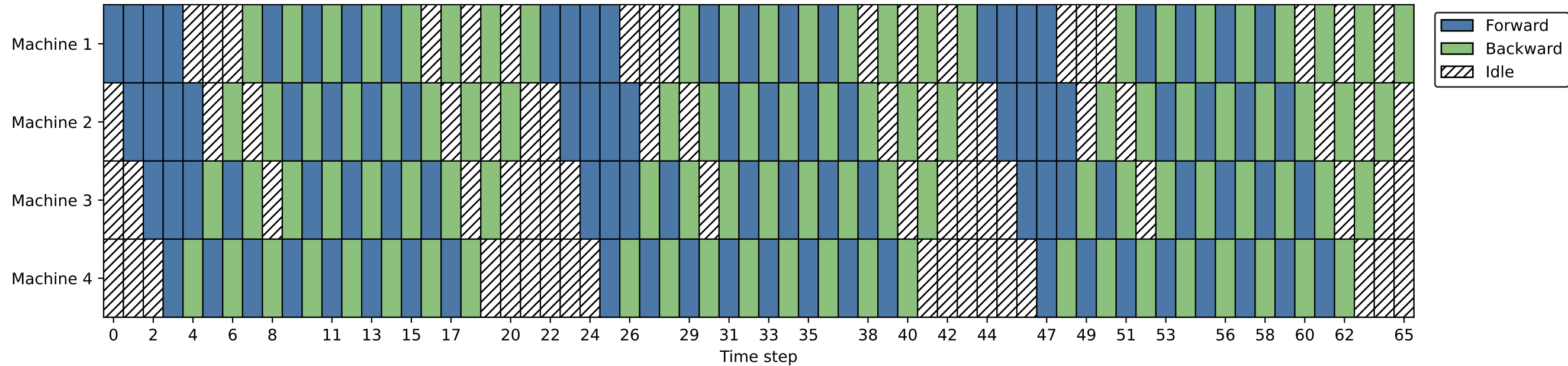
Local SGD pipeline Schedule ( H = 2 )
