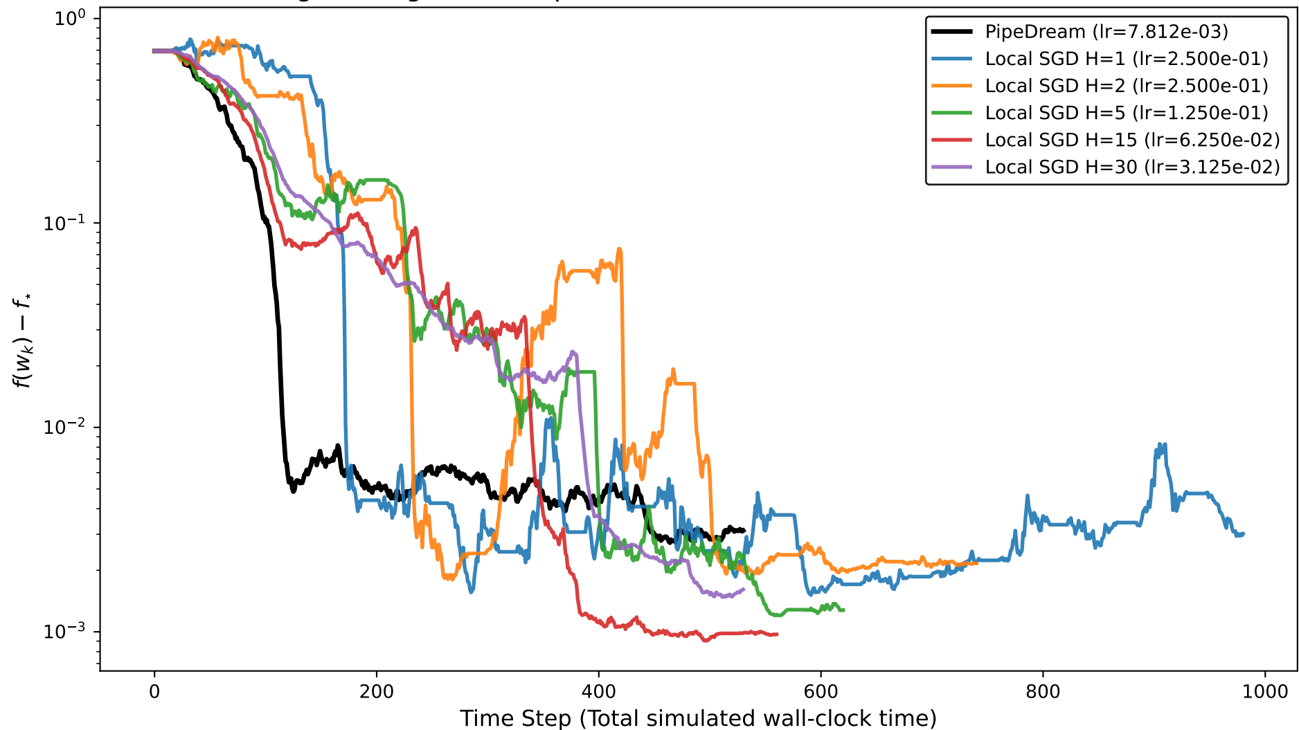
Logistic Regression: PipeDream vs. Local SGD (R=S=16 local runs)
