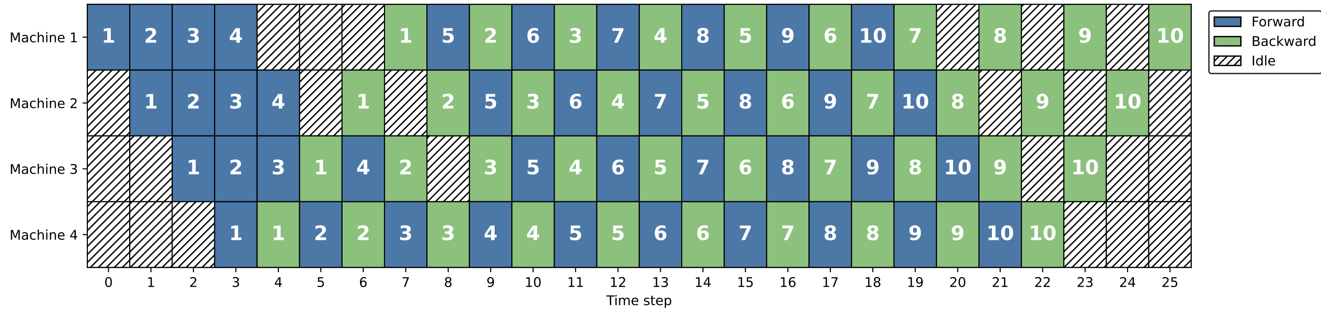
PipeDream-style 1F1B schedule
