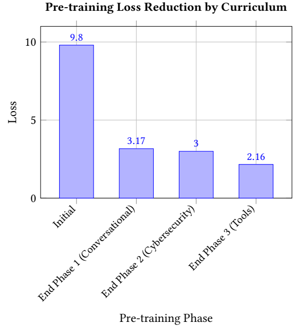
Figure 1: Validation loss monotonically decreases across the three curriculum pre-training phases. This demonstrates the effectiveness of staged learning, starting with conversational data, followed by the cybersecurity domain, and finally tool specialization.
