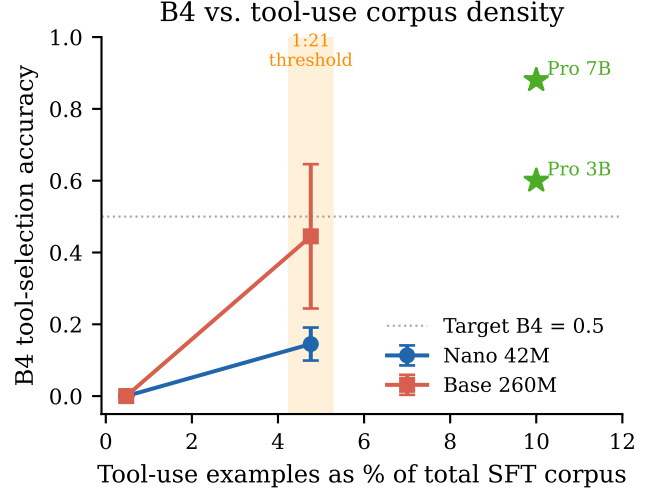
Figure 2: B4 tool-selection accuracy vs. tool-use corpus density (as % of total SFT examples). Error bars show \pm 1 std over N = 4 seeds. The density threshold between 1:211 and 1:21 shifts the first-token prior from prose to <|tool_call|> . Pro 3B and 7B are shown at their approximate SFT ratio (~1:10) for reference.
