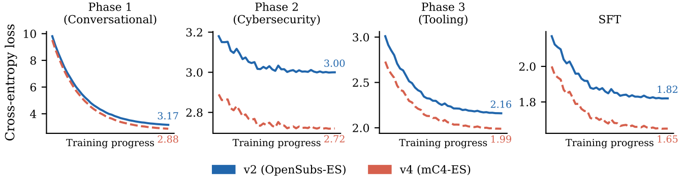
Figure 2: Training loss per phase for v2 (OpenSubtitles-ES bootstrap, solid) vs. v4 (mC4-ES bootstrap, dashed). v4 achieves lower loss in every post-Phase-1 phase, yet produces worse conversational behavior (B5: 6/10 vs. 7/10), illustrating the loss-vs-register inversion discussed in Section 9.
