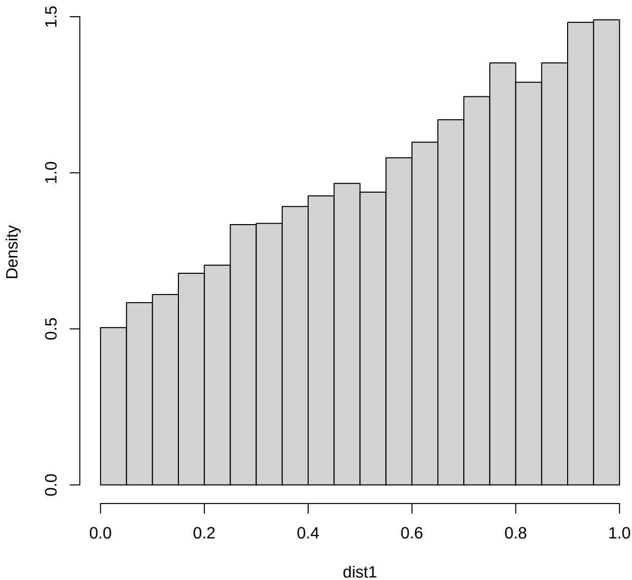
Histogram of dist1
