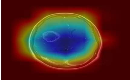
Grad-CAM
