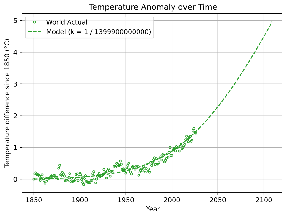
Figure 9: Temperature model compared to real world historical temperature anomaly, dataset from Our World in Data for years 1850–2026. mean error = <0.0003°C, error stdev = 0.1259°C
