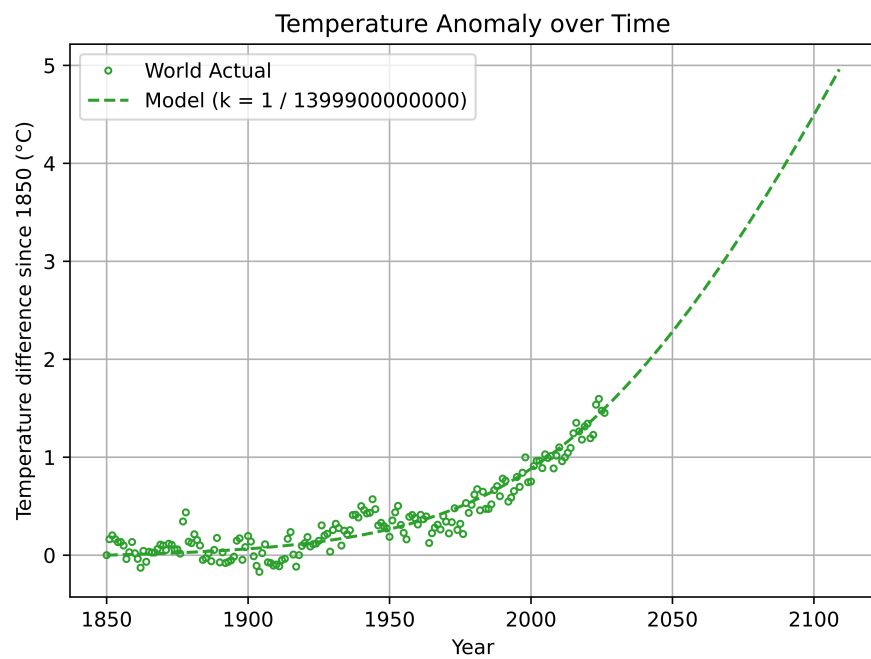
Figure 9: Temperature model compared to real world historical temperature anomaly, dataset from Our World in Data for years 1850–2026. mean error \approx 0^\circ\text{C} , error stdev = 0.1259^\circ\text{C}
