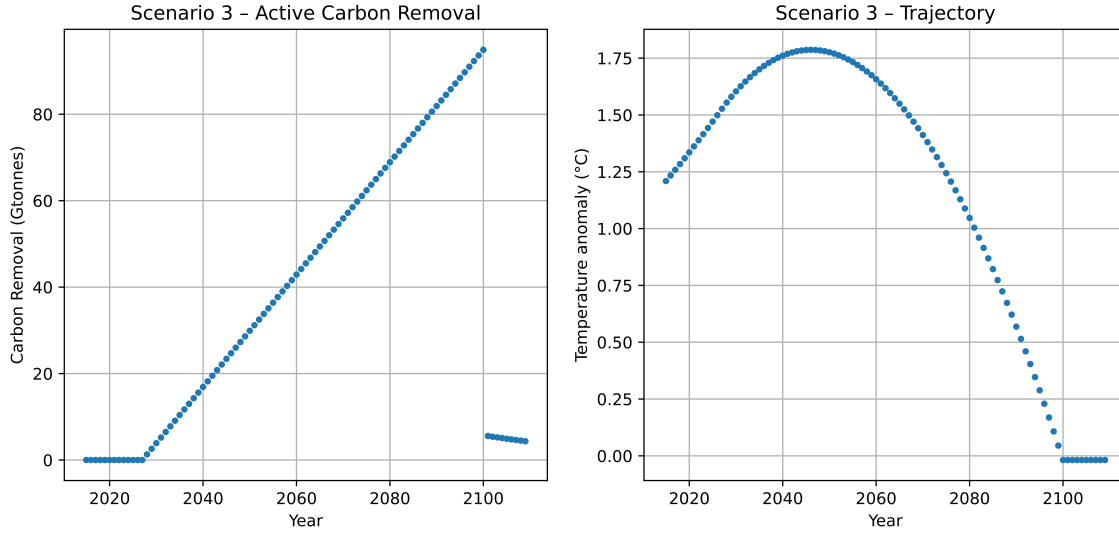
Figure 3: Scenario 3 active \text{CO}_2 removal and resulting temperature projections
