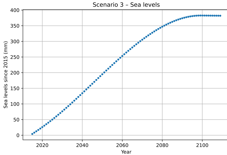
Figure 4: Scenario 3 model sea levels since 2015
