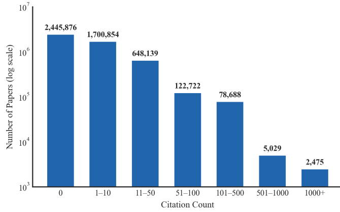
Figure 5: Citation distribution across the 5,003,783 AI papers in the corpus, shown on a log scale.
