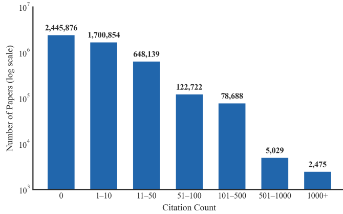
Figure 5: Citation distribution across the 5M+ AI papers in the corpus, shown on a log scale.
