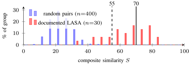
Fig. 6. Score distributions for documented confusable pairs and random corpus pairs, binned at width 5 and normalised within each group so that the two very different sample sizes are comparable. The distributions are almost disjoint, which is what a ROC AUC of 0.997 means concretely, and the residual overlap sits entirely below the review line.
