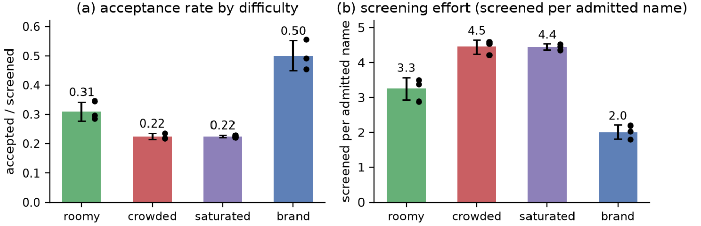
Fig. 9. Acceptance rate and screening effort by difficulty stratum across the three seeds (bars: mean; whiskers: standard deviation; dots: per-seed values). The seed spread is an order of magnitude larger for brand than for generic, because brand shortlists are anchored by what the proposers draw in a given seed while stem-governed ones are anchored by the mandated ending itself.
