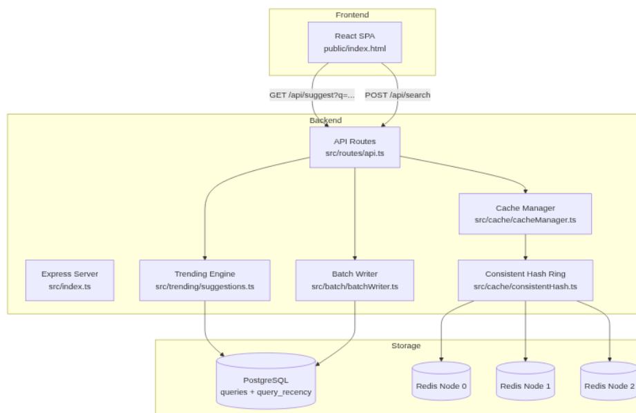
Architecture Diagram
