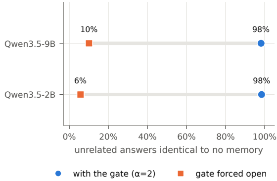
Figure 6: Unrelated replies identical to no memory, at \alpha=2 , with the gate and with the gate forced open.
