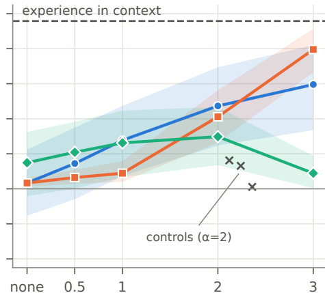
Qwen3.5-9B
