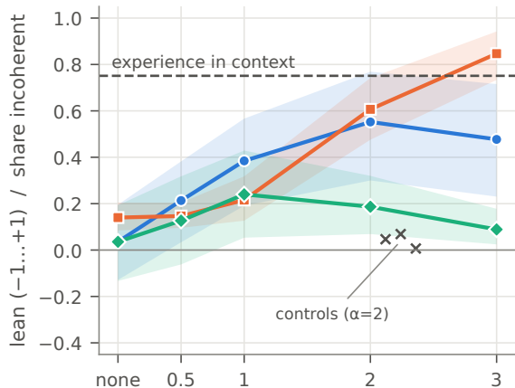
Qwen3.5-2B
