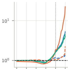
T850
