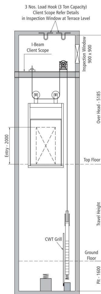
Lift Well Section View
