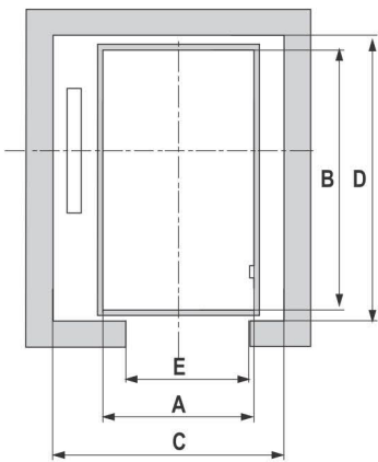
Mini Gearless Machine For Home Lift
