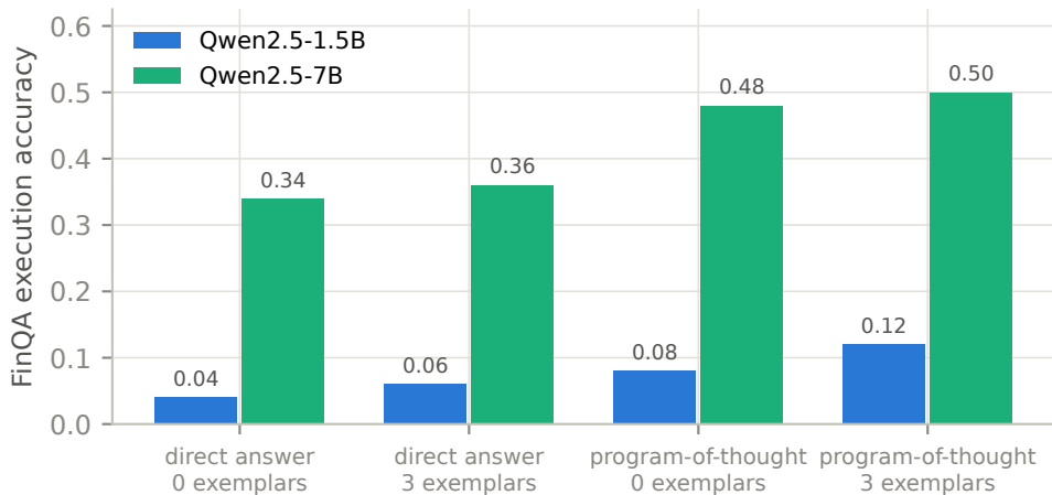
Generation ablation: prompt form \times exemplars, at two model sizes
