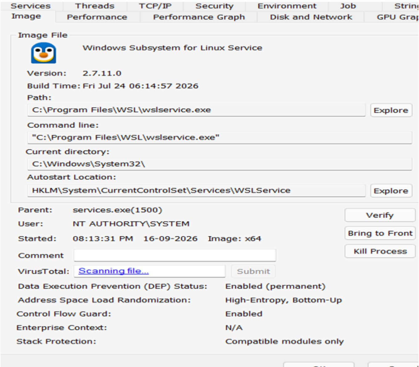
Figure 2.1: Inspecting suspicious process properties.
