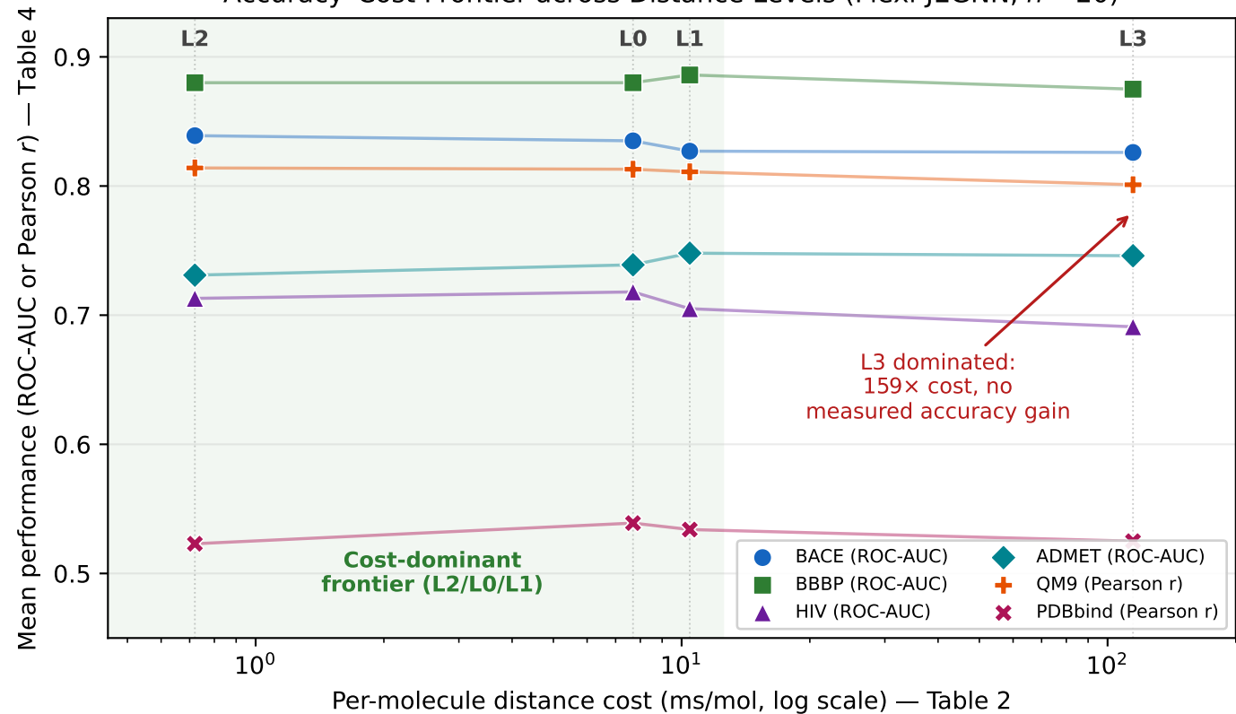
Accuracy-Cost Frontier across Distance Levels (Flexi-JEGNN, n = 20 )
