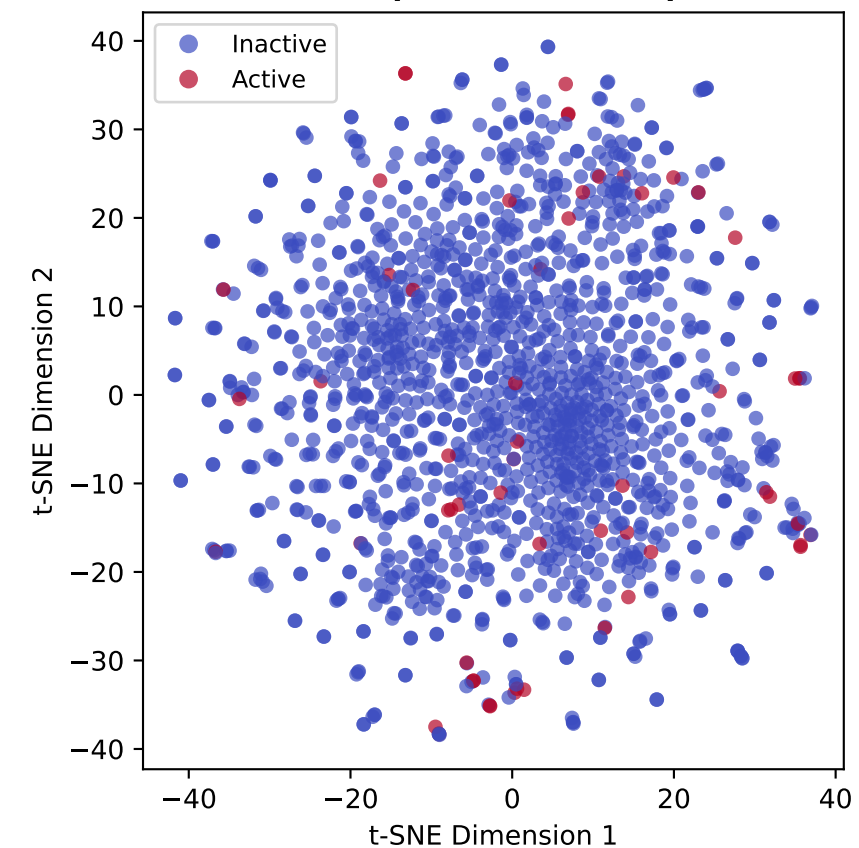
ADMET (Classification)
