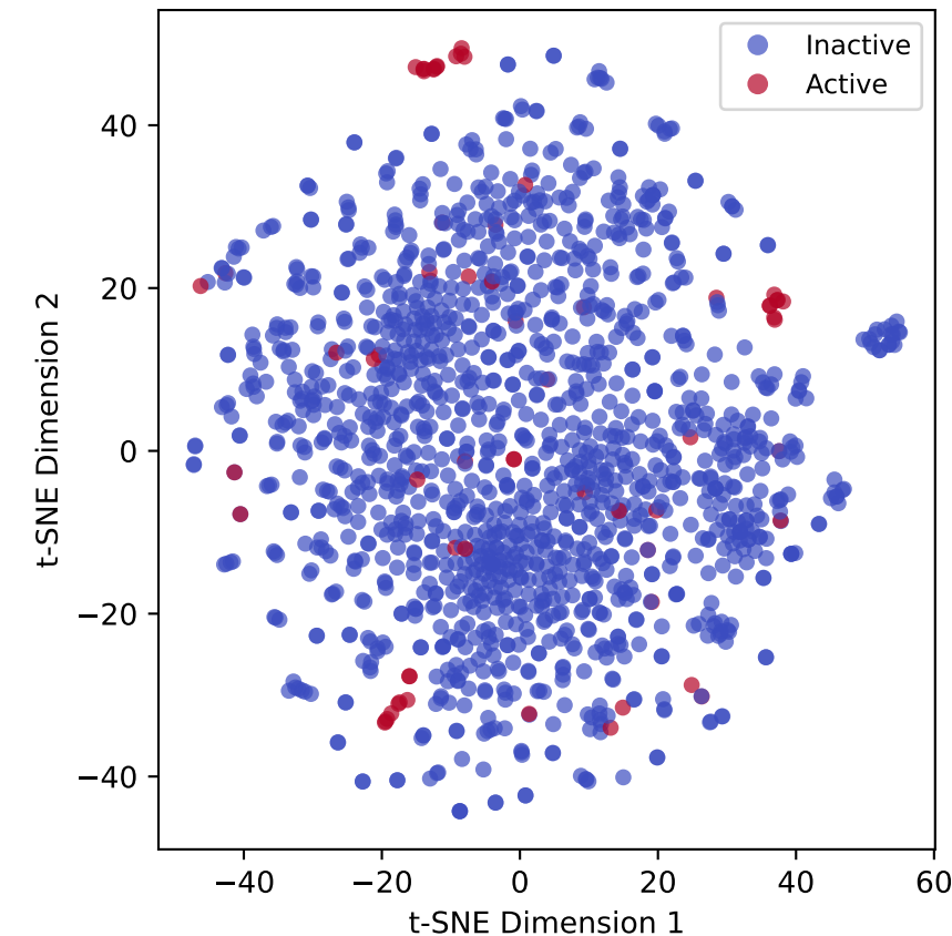
ADMET (Classification)
