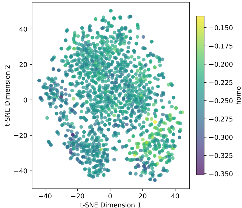
QM9 (Regression)
