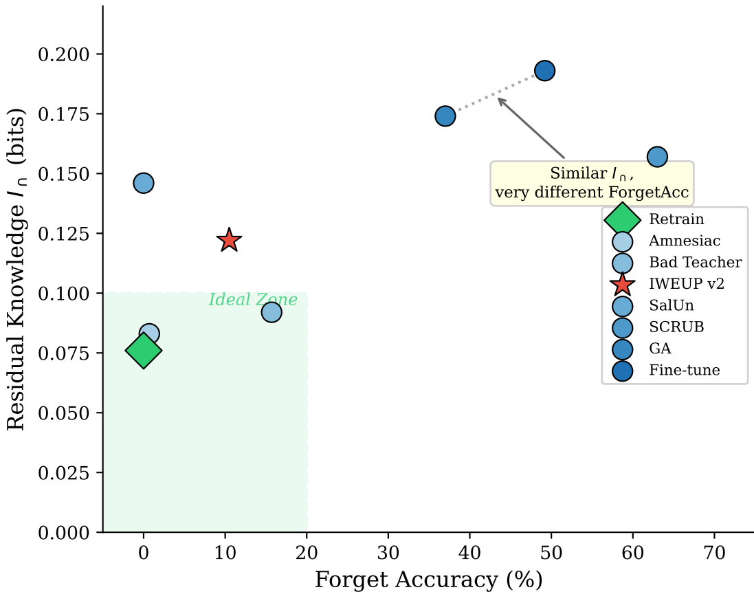
I_n vs. Forget Accuracy — Metric Disagreement
