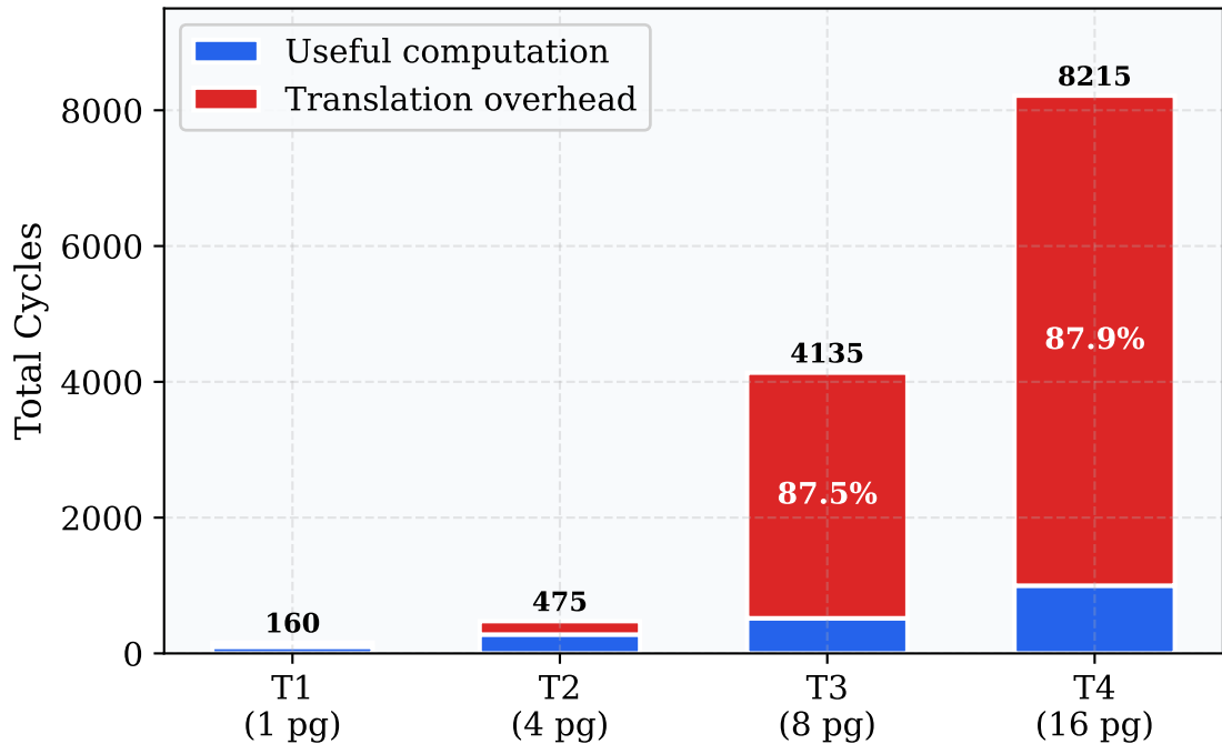
Cycle Breakdown: Useful Computation vs Translation Overhead
