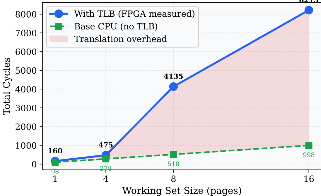
Execution Time: TLB-Enabled vs Base CPU
