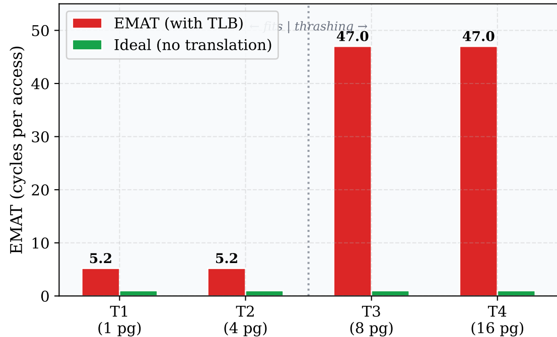
Effective Memory Access Time
