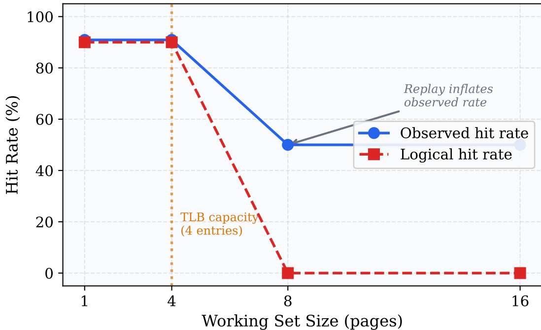
TLB Hit Rate: Observed vs Logical
