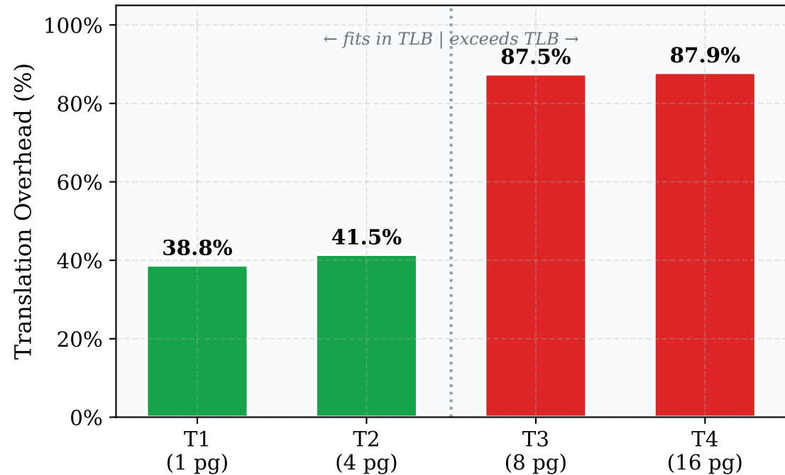
Address Translation Overhead vs Working Set Size
