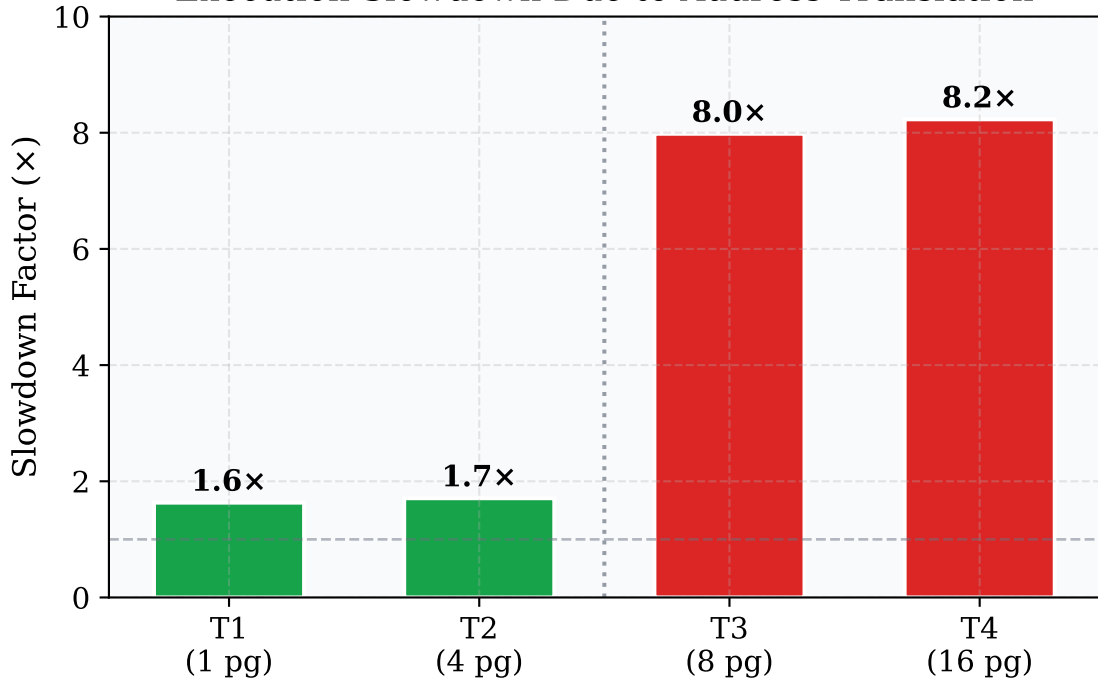
Execution Slowdown Due to Address Translation
