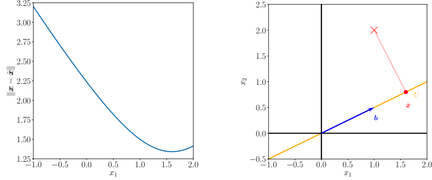
(a) Distances \|\mathbf{x} - \tilde{\mathbf{x}}\| for some \tilde{\mathbf{x}} = z_1 \mathbf{b} \in U = \text{span}[\mathbf{b}] ; see panel (b) for the setting.
