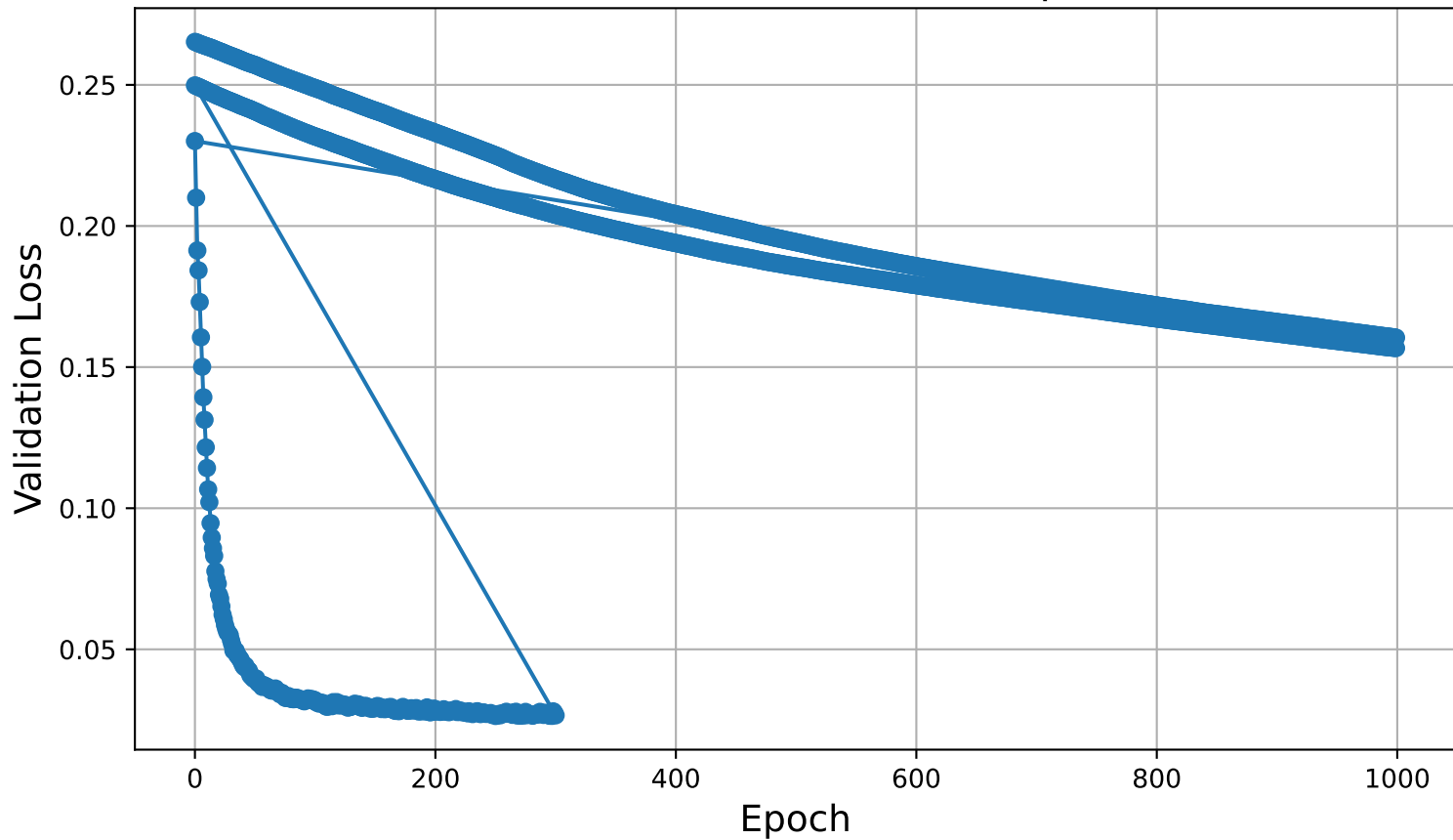
Trial 0 - Validation Loss vs. Epoch
