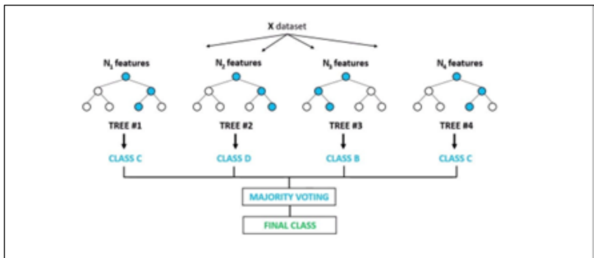
Fig 2.5 Random Forest Classifier
