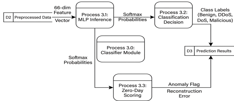
Fig 4.7 DFD Level 2 diagram for Classifier Data Module
