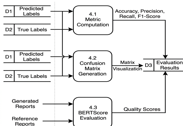
Fig 4.8 DFD Level 2 diagram for Evaluation module
