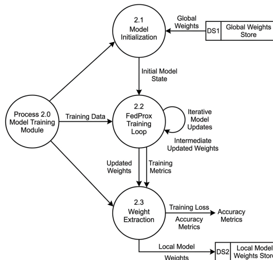
Fig 4.6 DFD Level 2 diagram for Trained Model
