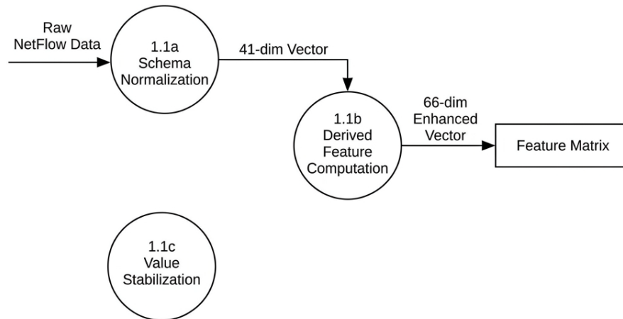
Fig 4.5 DFD Level 2 diagram for Feature Extraction
