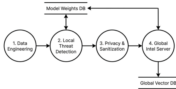
Fig 4.3 DFD Level 1 diagram
