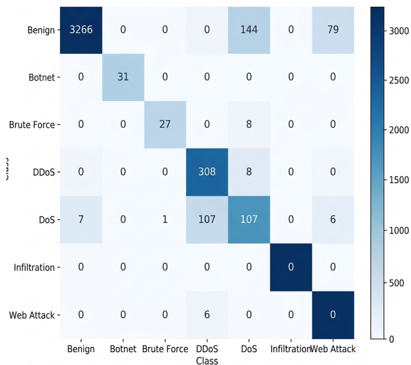
Fig 8.1 Confusion Matrix
