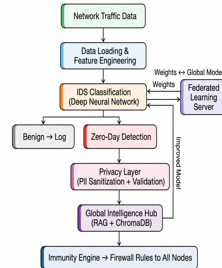
Fig 4.1 System Architecture
