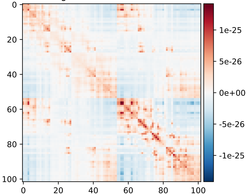
Magnetometers covariance
